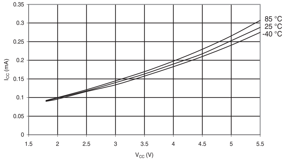
Figure 29-56. ATmega48PA: Idle Supply Current vs. V_{CC} (Internal RC Oscillator, 1 MHz)
