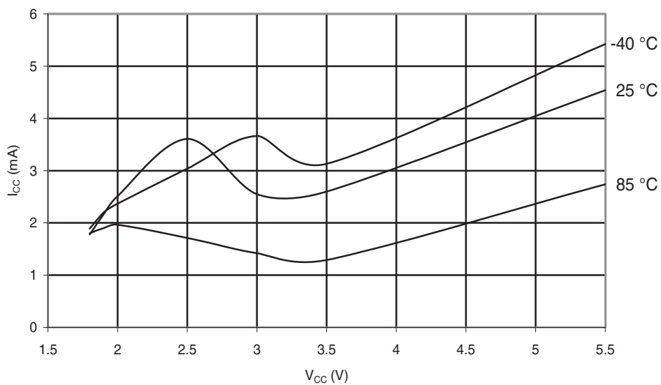
Figure 29-91. ATmega48PA: Programming Current vs. V_{CC}
