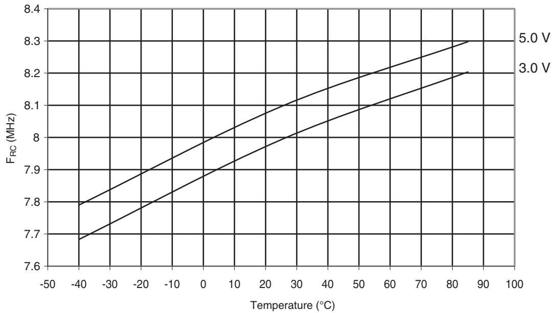
Figure 29-320. ATmega328: Calibrated 8 MHz RC Oscillator Frequency vs. Temperature
