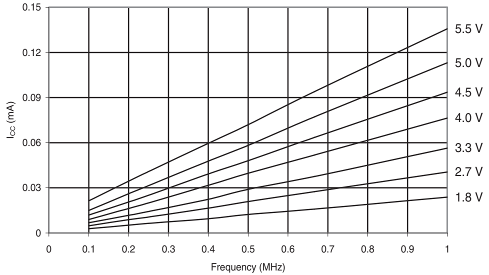
Figure 29-241. ATmega168PA: Idle Supply Current vs. Low Frequency (0.1-1.0 MHz)
