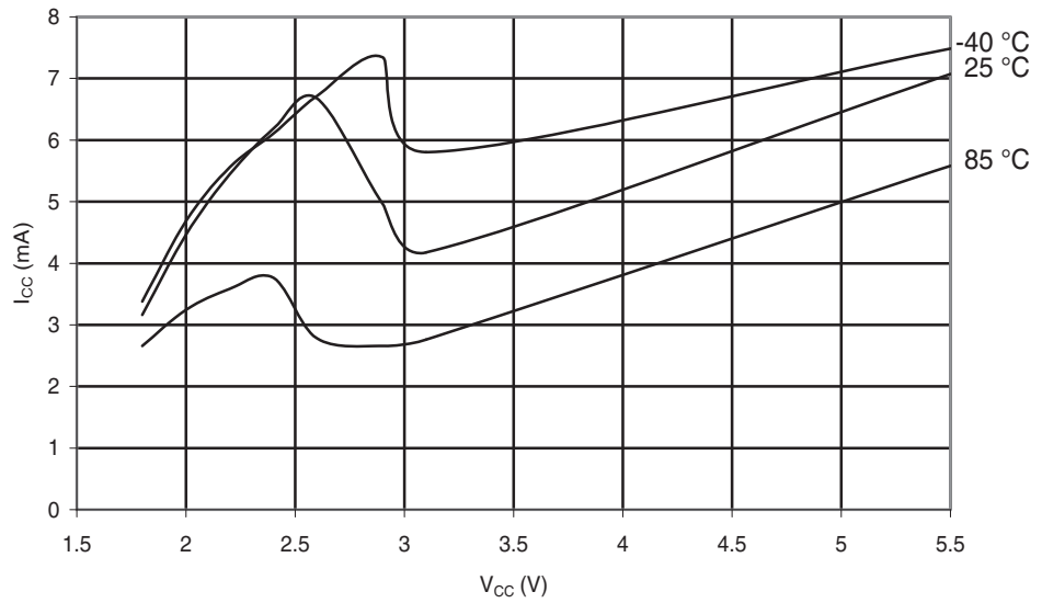
Figure 29-138. ATmega88A: Programming Current vs. V_{CC}
