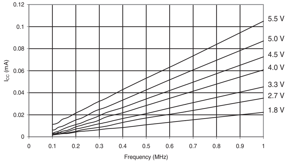
Figure 29-186. ATmega88PA: Reset Supply Current vs. Low Frequency (0.1 - 1.0 MHz)
