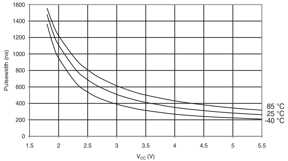
Figure 29-94. ATmega48PA: Minimum Reset Pulse width vs. V_{CC}
