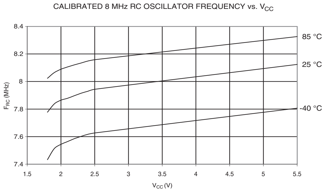
Figure 29-319. ATmega328: Calibrated 8 MHz RC Oscillator Frequency vs. V_{CC}
