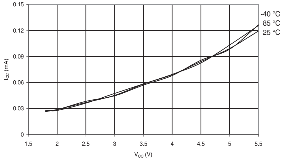
Figure 29-191. ATmega168A: Active Supply Current vs. V_{CC} (Internal RC Oscillator, 128 kHz)
