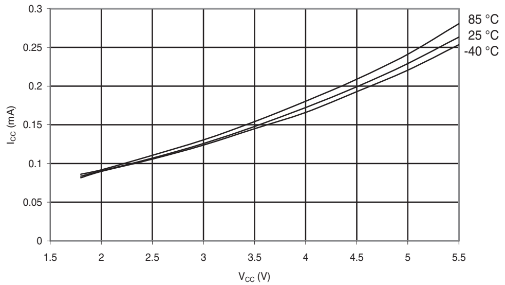
Figure 29-244. ATmega168PA: Idle Supply Current vs. V_{CC} (Internal RC Oscillator, 1 MHz)
