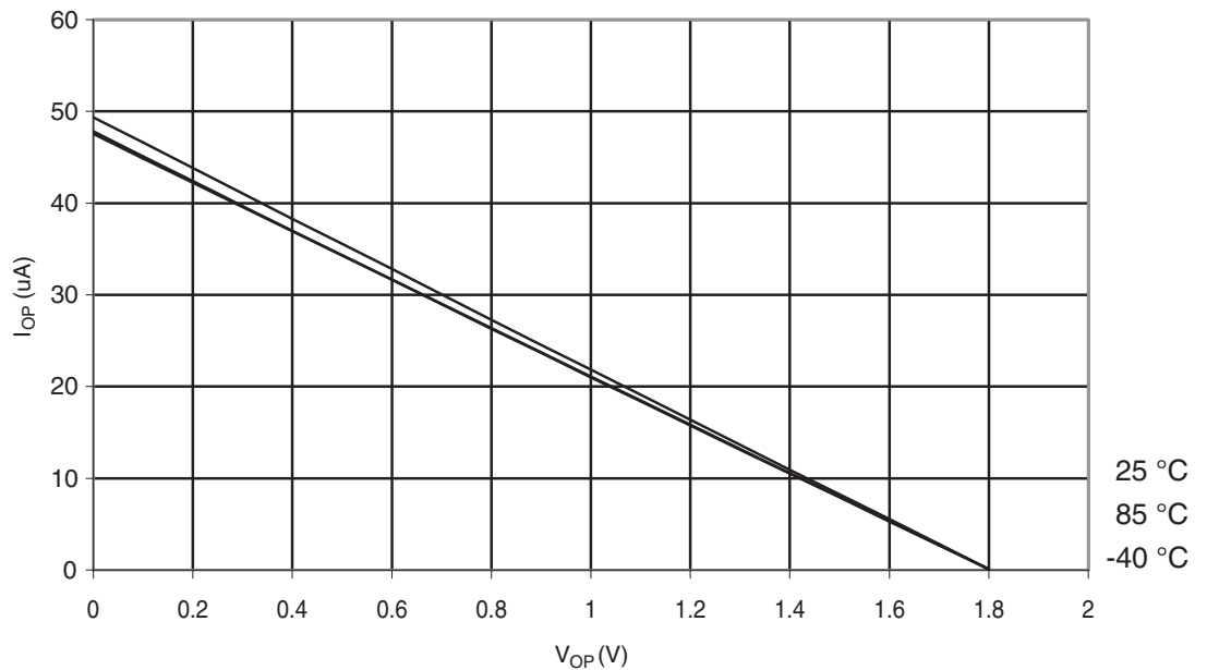
Figure 29-297. ATmega328: I/O Pin Pull-up Resistor Current vs. Input Voltage (V CC = 1.8 V)
