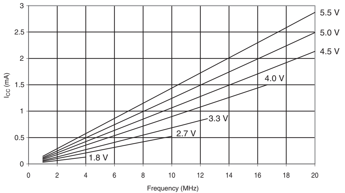
Figure 29-375. ATmega328P: Reset Supply Current vs. Frequency (1 - 20 MHz)
