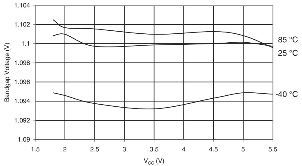
Figure 29-34. ATmega48A: Bandgap Voltage vs. V_{CC}
