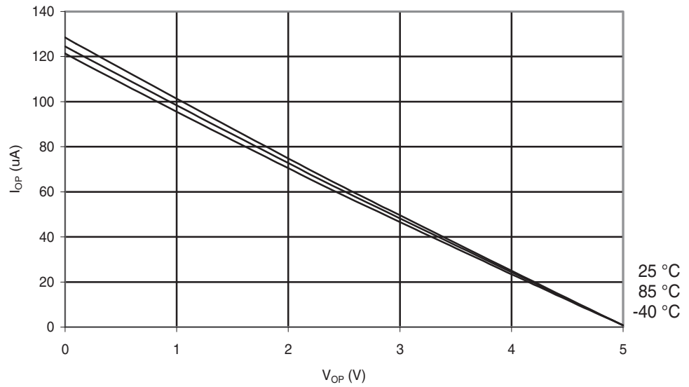
Figure 29-64. ATmega48PA: I/O Pin Pull-up Resistor Current vs. Input Voltage ( V_{CC} = 5\text{ V} )
