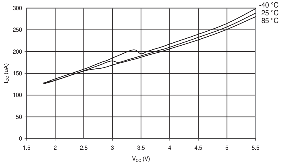
Figure 29-181. ATmega88PA: ADC Current vs. V_{CC} (AREF = AV_{CC} )
