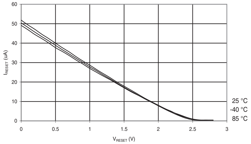
Figure 29-19. ATmega48A: Reset Pull-up Resistor Current vs. Reset Pin Voltage ( V_{CC} = 2.7\text{ V} )
