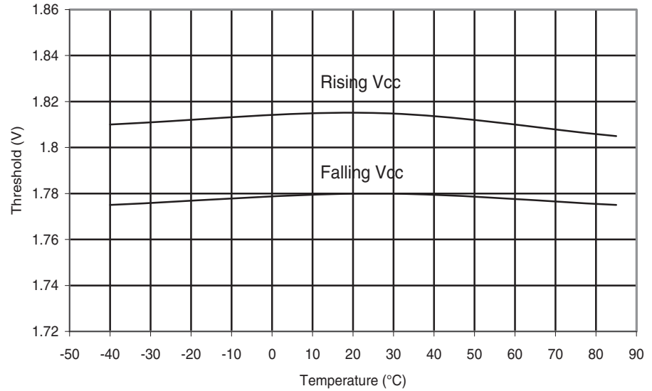
Figure 29-219. ATmega168A: BOD Thresholds vs. Temperature (BODLEVEL is 1.8 V)
