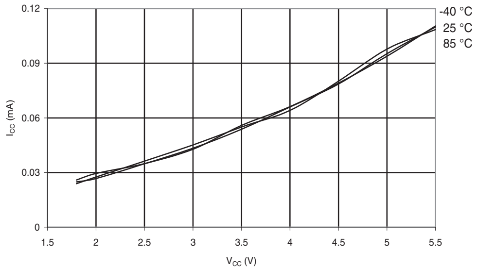
Figure 29-144. ATmega88PA: Active Supply Current vs. V_{CC} (Internal RC Oscillator, 128 kHz)
